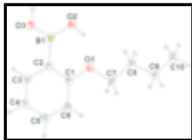
Fig. 1. The molecular structure of (I). Displacement ellipsoids are drawn at the 50% probability level.
