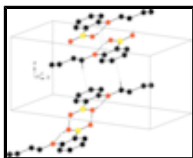
Fig. 2. The crystal packing in (I) showing hydrogen-bonding, C—H...π and π-π interactions as dashed lines.
